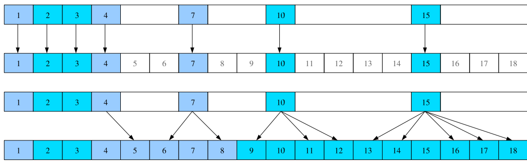
Figure 5.5: Generation of the warm-start iterate.
